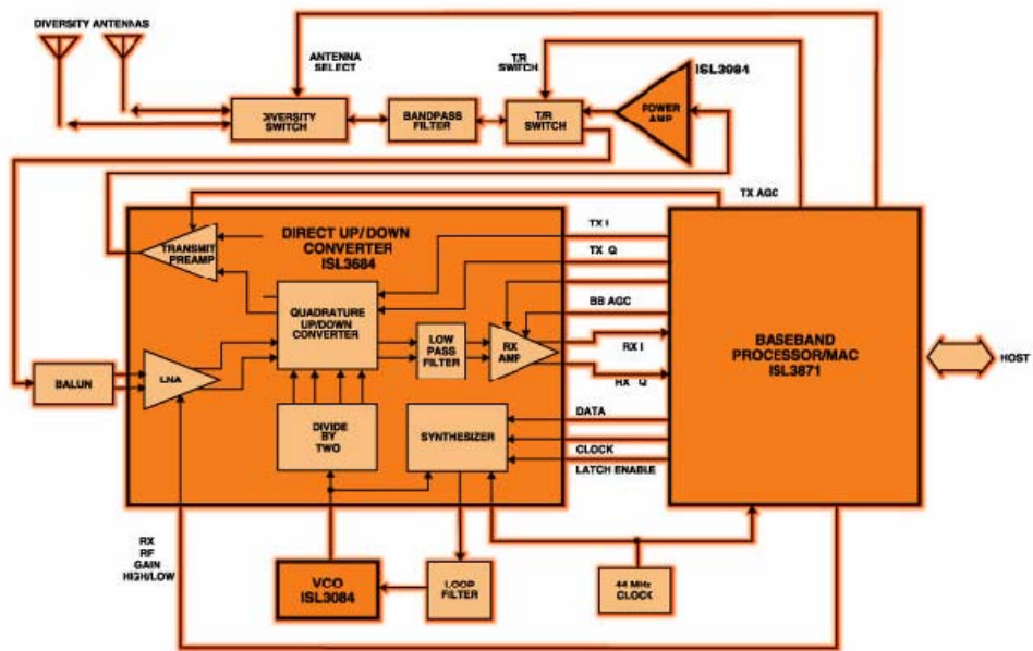
Fig.1 PRISM3.0 USB Radio Block Diagram
