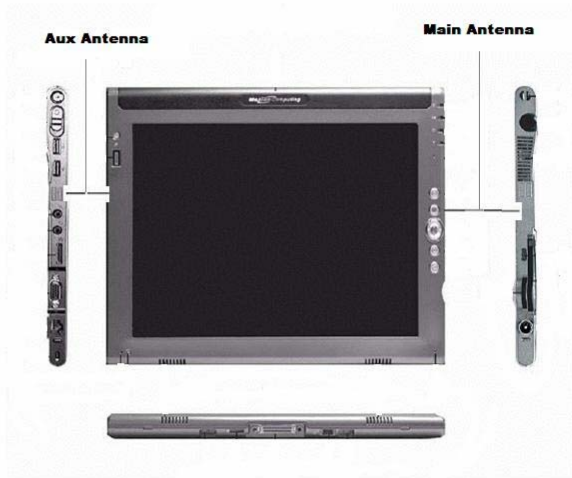
Figure 2: Aux (left side) and Main (right side) Antenna location
