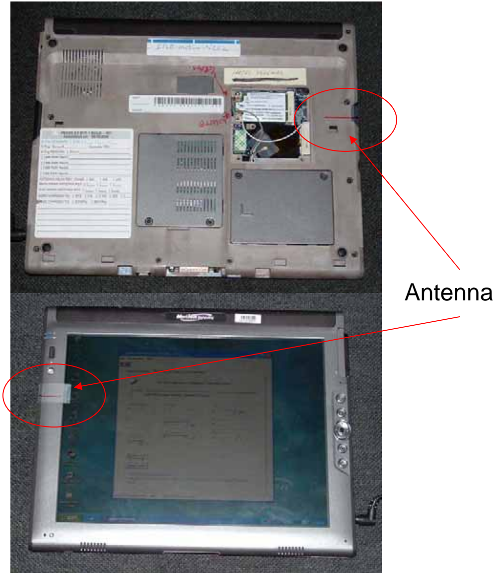
Pecos II Main Antenna Location
