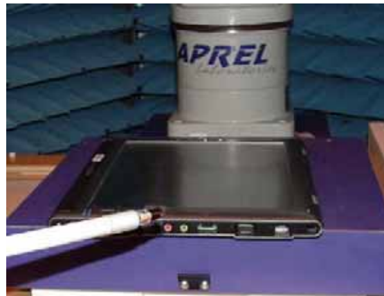
Sniffer Probe Antenna Location
