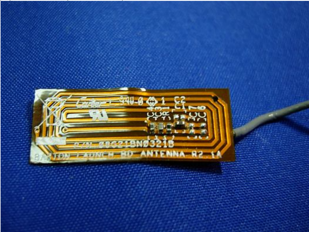
(22) EUT Photo – (RF ID Antenna)
