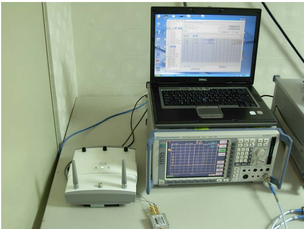
DFS Set-up Photo: Master and Spectrum Analyzer
