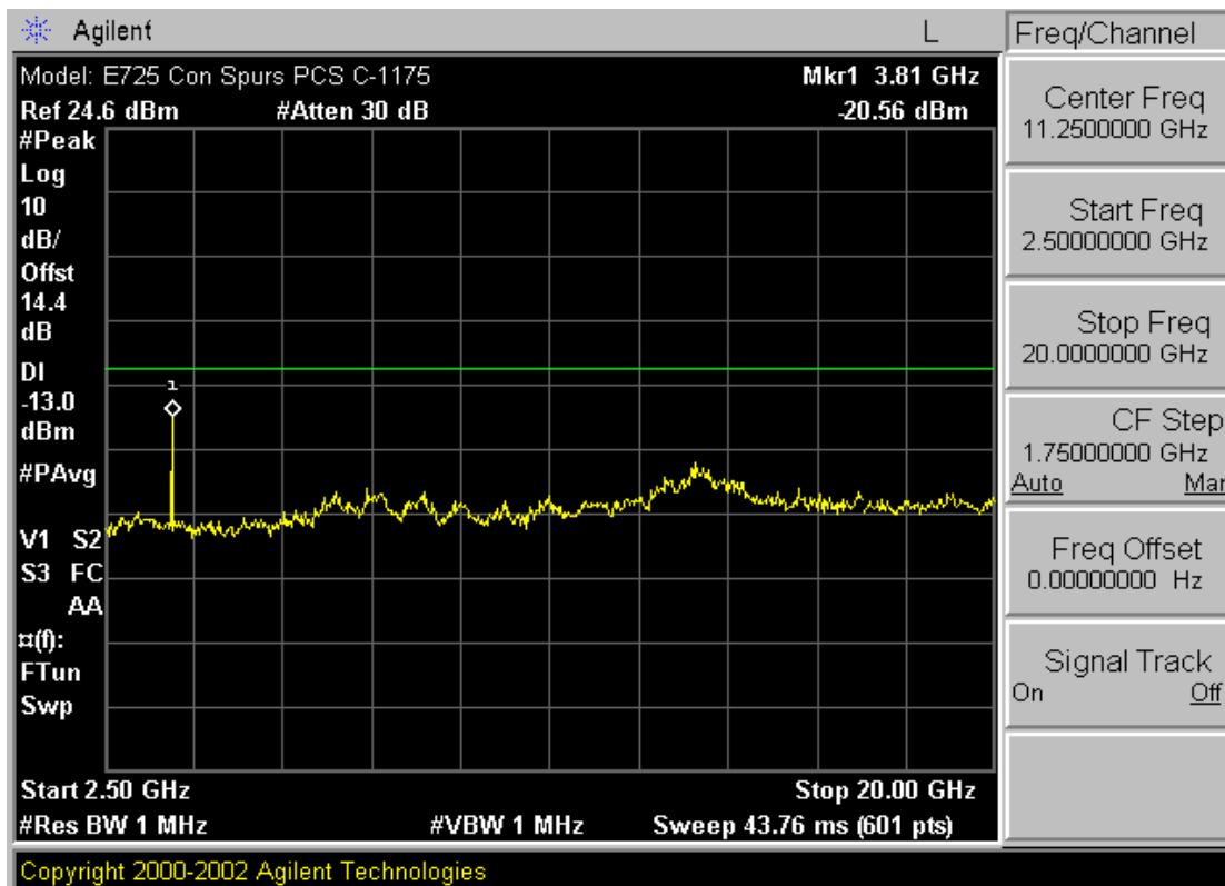
Plot A-22. Conducted Spurious Plot (PCS CDMA Mode – Ch. 1175)
