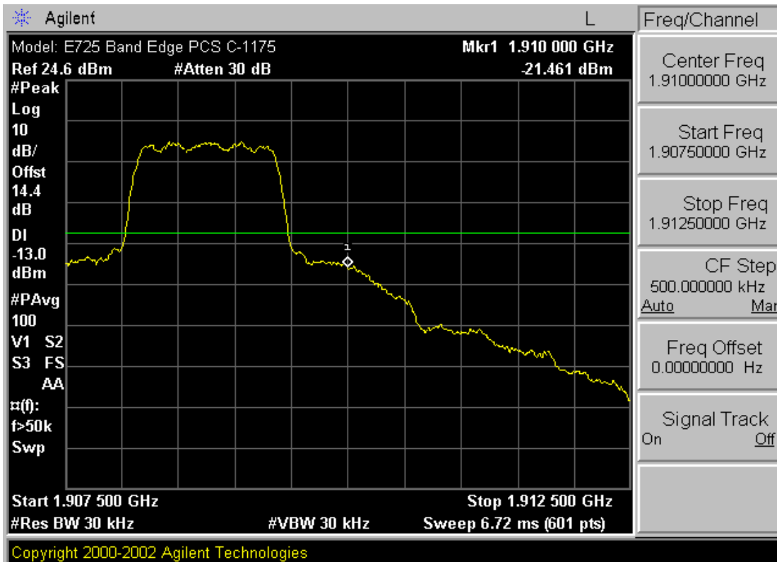
Plot A-23. Band Edge Plot (PCS CDMA Mode – Ch. 1175)
