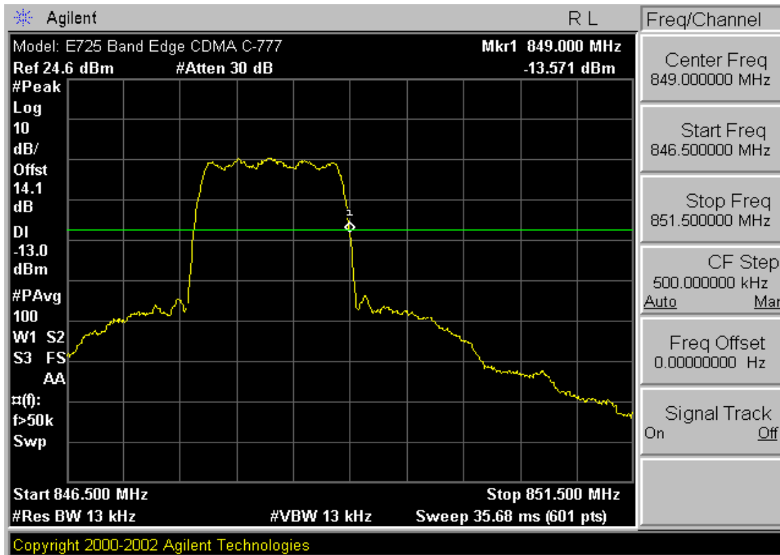
Plot A-11. Band Edge Plot (Cellular CDMA Mode – Ch. 777)
