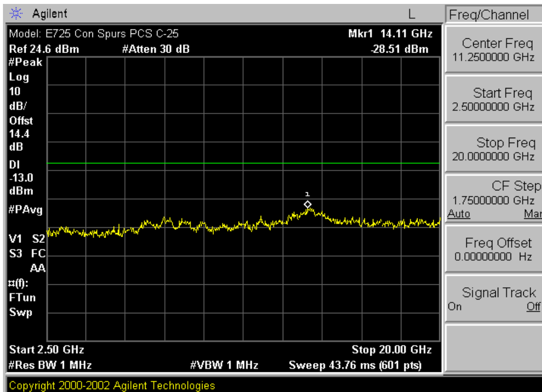
Plot A-14. Conducted Spurious Plot (PCS CDMA Mode – Ch. 25)
