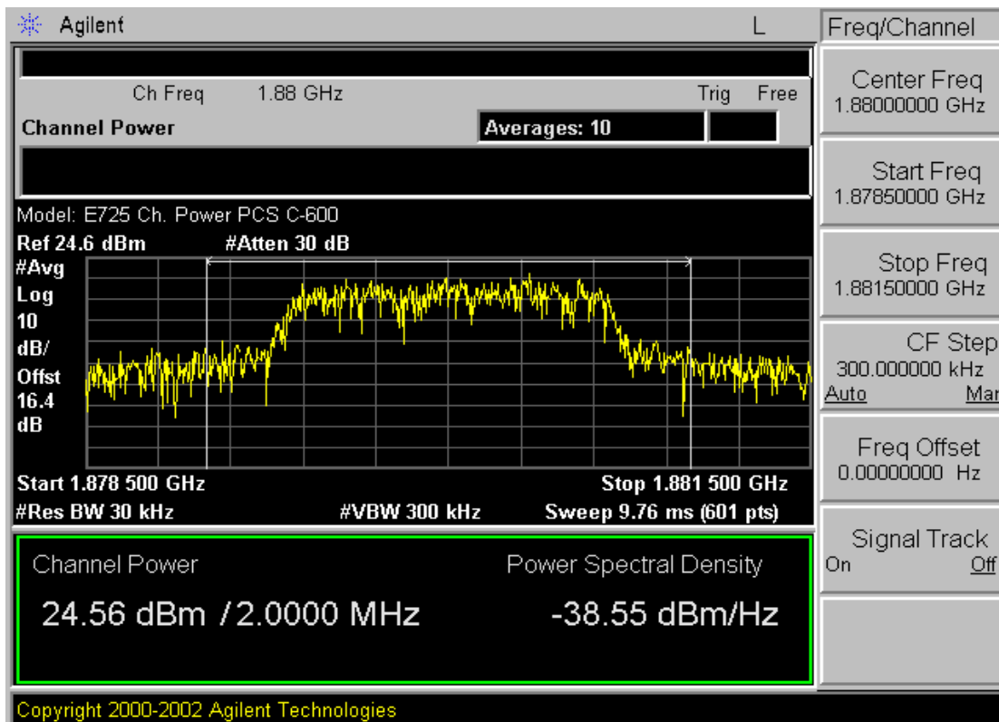
Plot A-20. Channel Power Plot (PCS CDMA Mode – Ch. 600)
