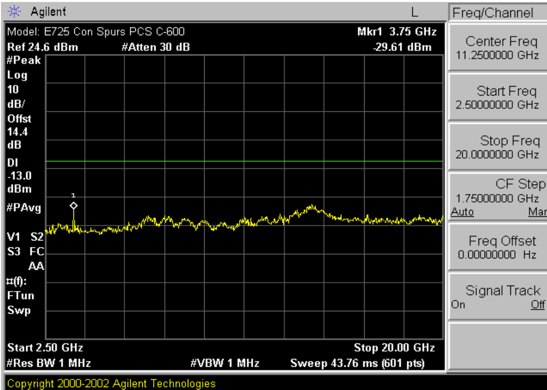
Plot A-18. Conducted Spurious Plot (PCS CDMA Mode – Ch. 600)
