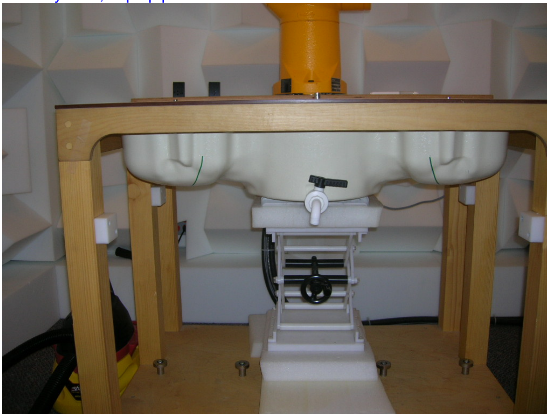
2. Body SAR, Laptop position.
