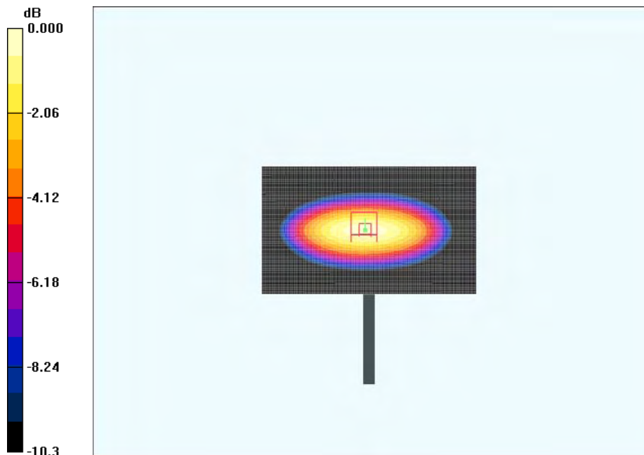
835 MHz System Validation with Body Tissue
