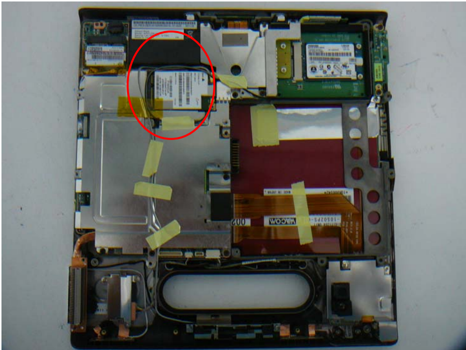
WWAN Module built into the Tablet PC (Motion CFT-003)
