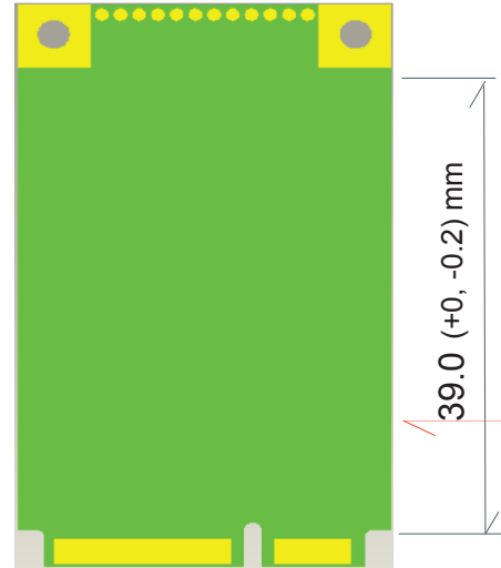
Module Bottom View (backside)
