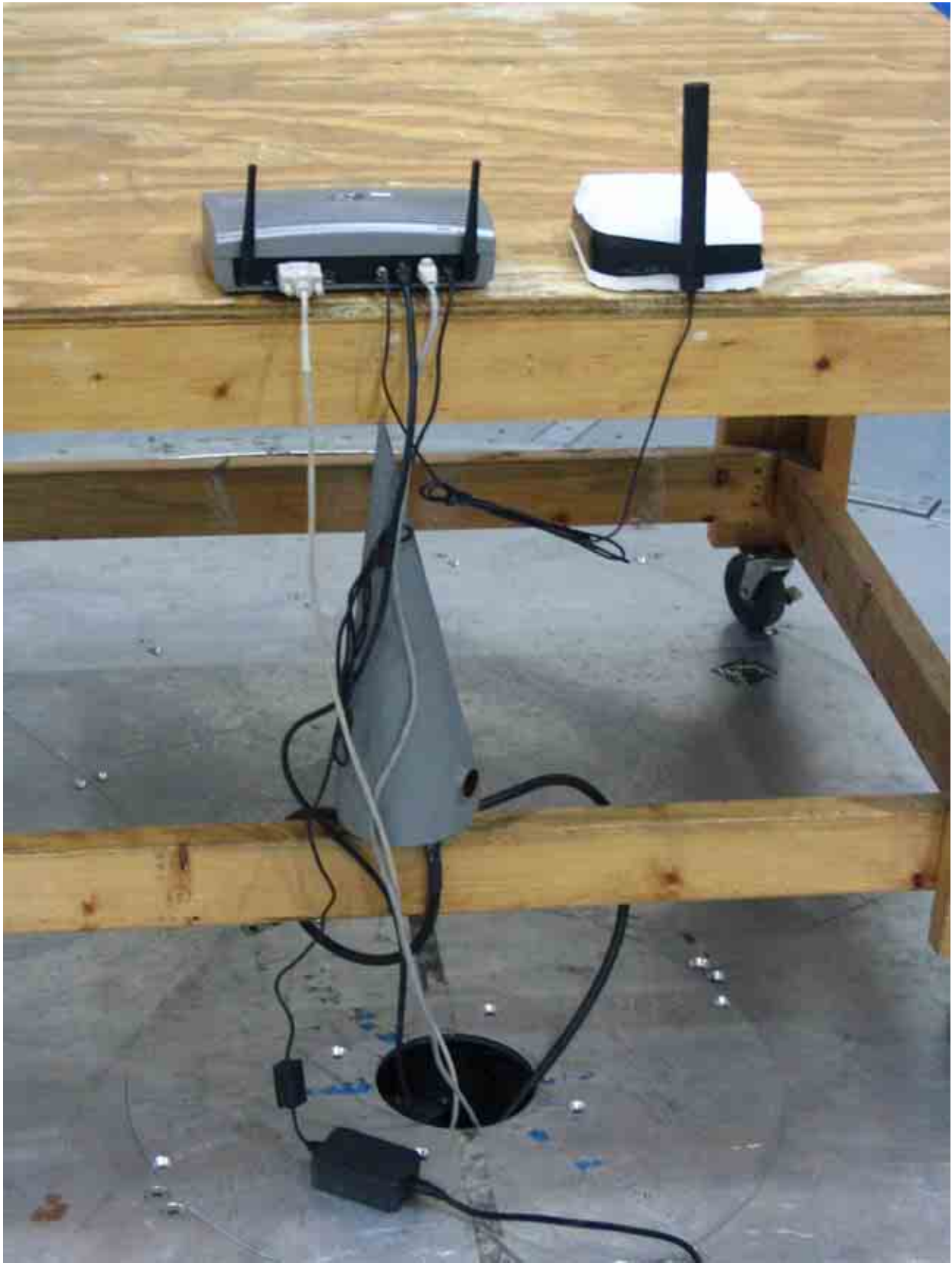
Figure 4: Radiated Emissions Testing (Back)
