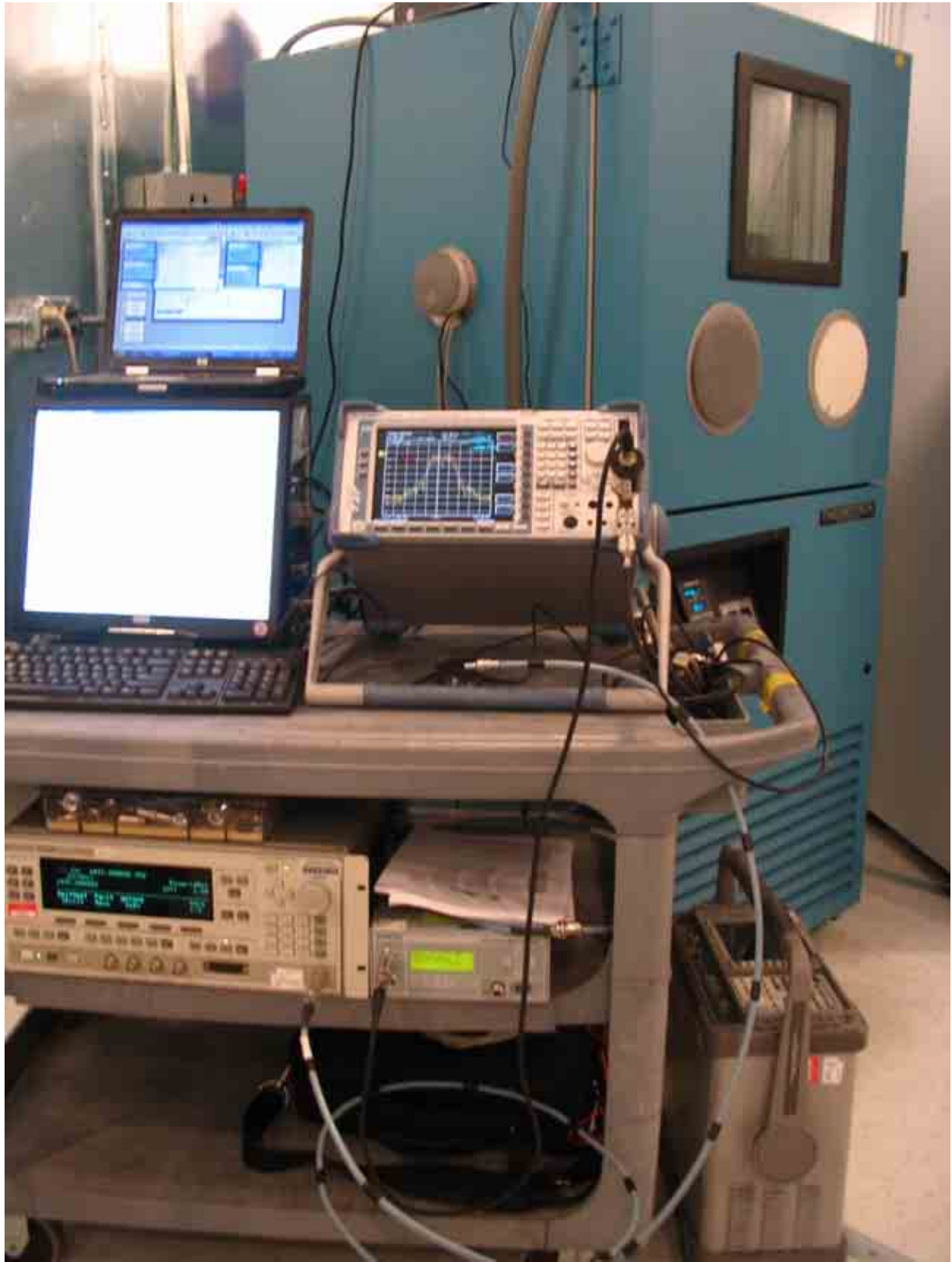
Figure 6: Frequency Stability Testing (Test Equipment Outside Chamber)
