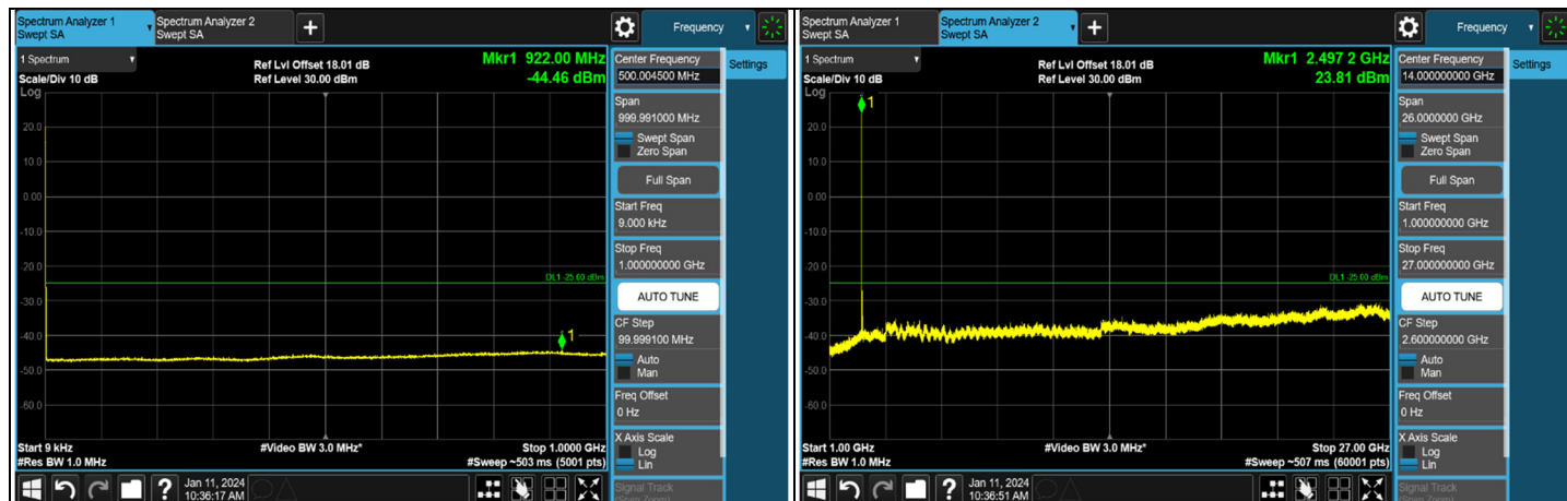
Channel 507204 (2536.02 MHz)
