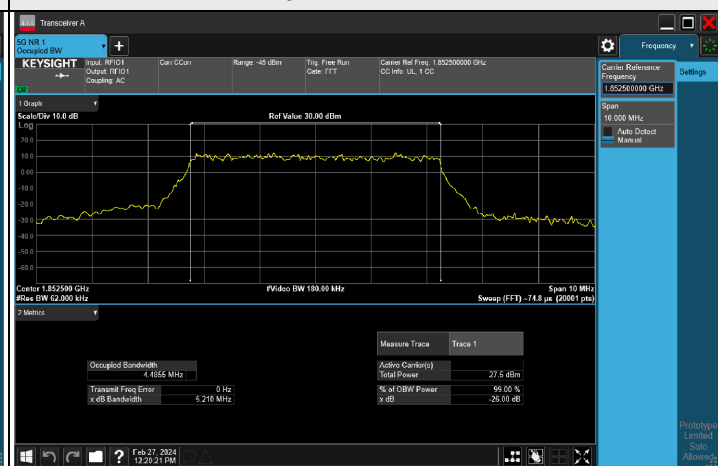
16QAM CH 370500 (1852.5 MHz)
