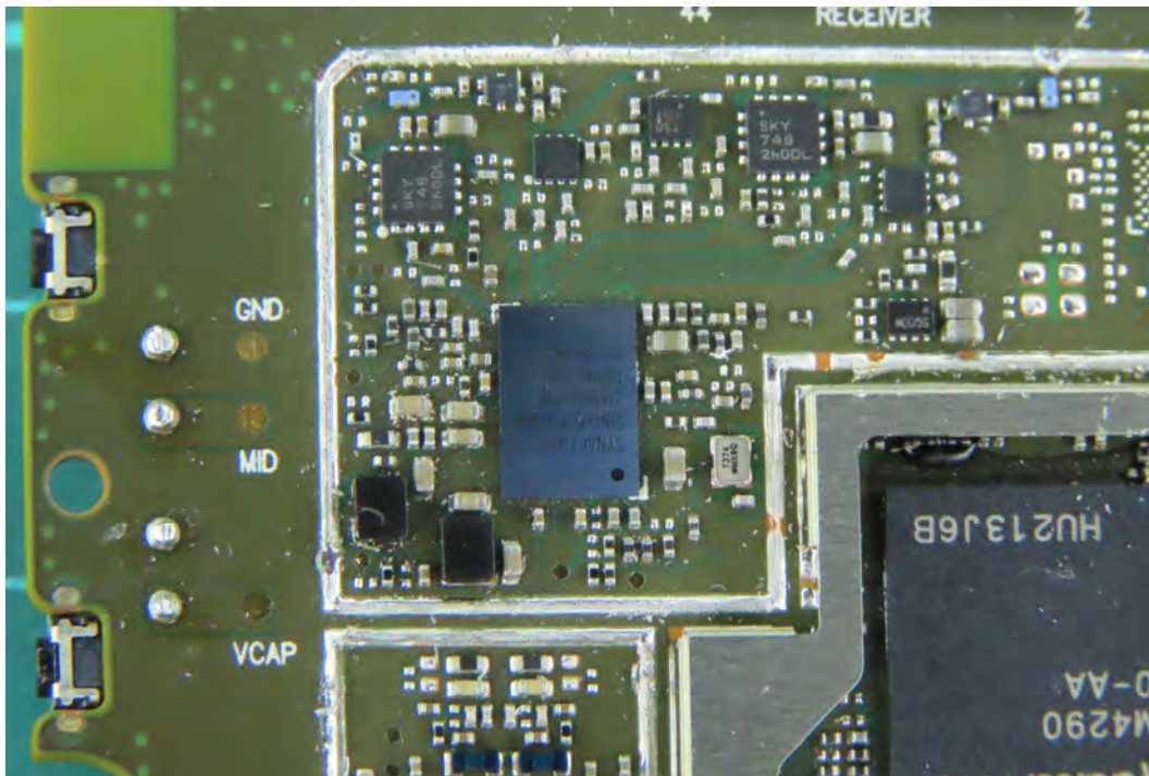
(26) EUT Photo
