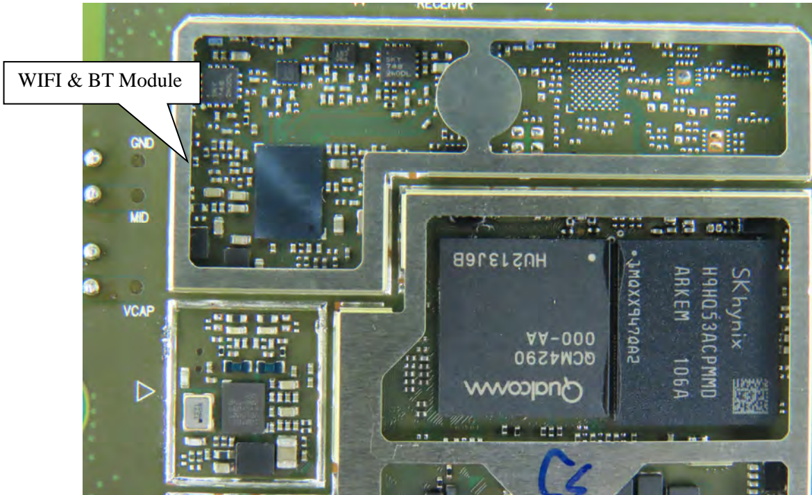
(25) EUT Photo
