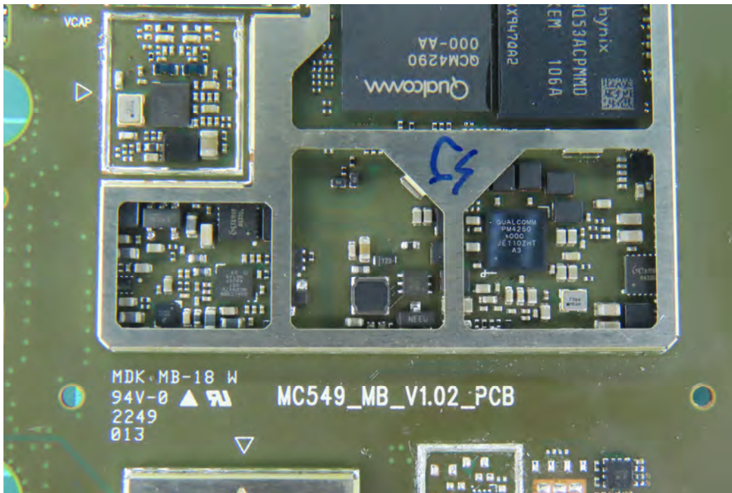
(28) EUT Photo
