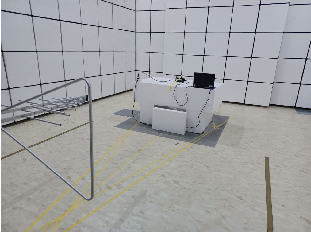
Radiated Test
