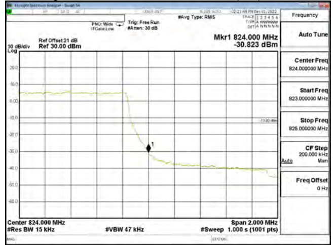
Bandedge B26 1.4 M CH26783 QPSK(6,0)
