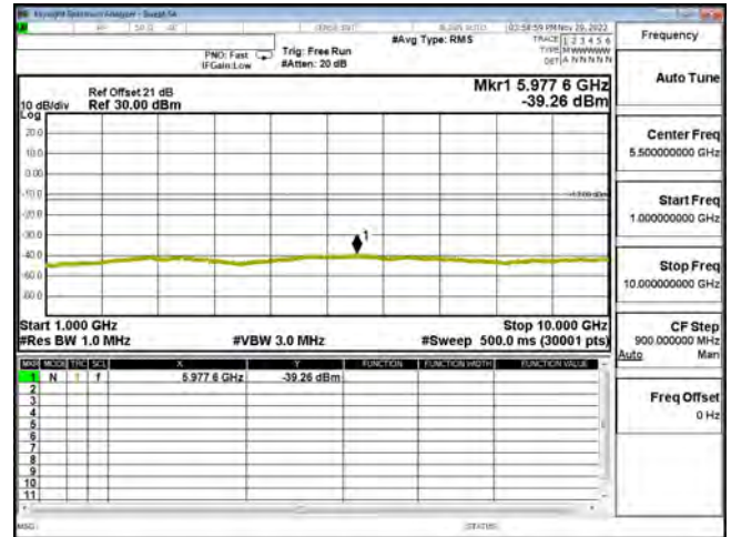
CSE B26 10 M CH2670 QPSK(1,0) 1 G-10 G
