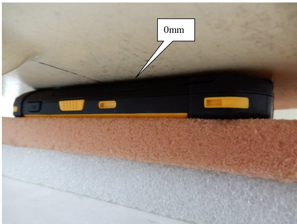
EUT Back – Limb SAR
