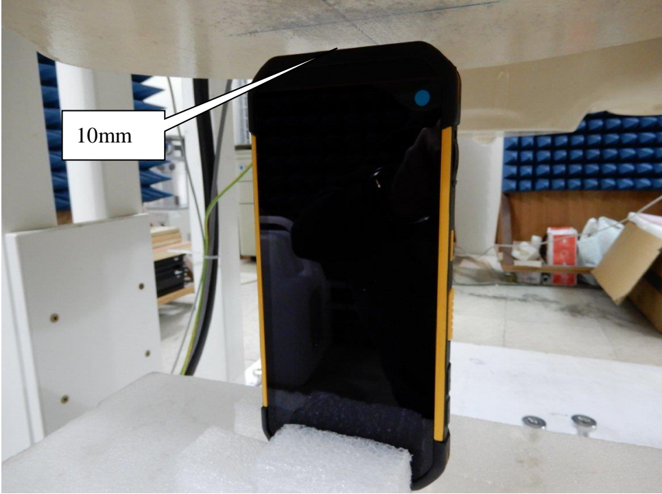
EUT Bottom – Body SAR
