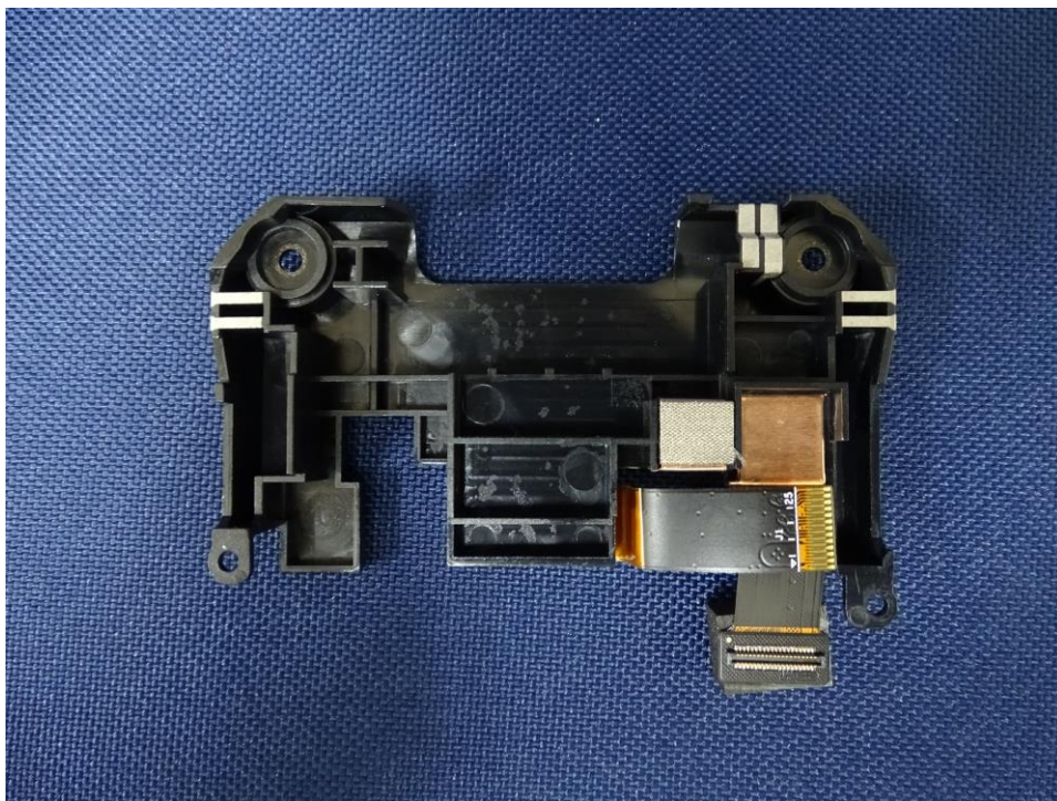
(16) EUT Photo - WWAN Aux Antenna
