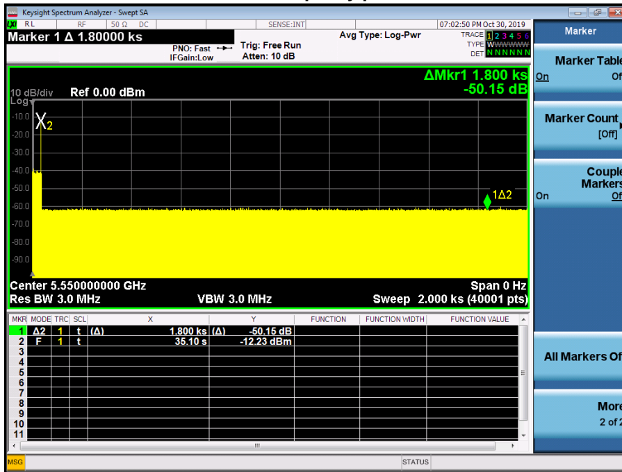
TX 11n (HT40) Mode Non-Occupancy period
