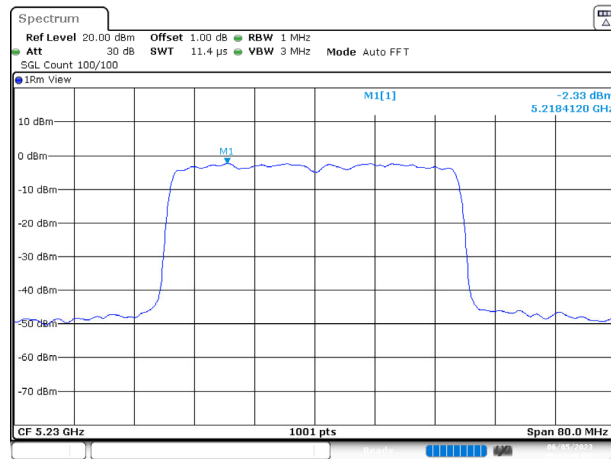
Channel 46
