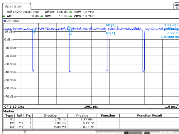
802.11ax-40 MHz
