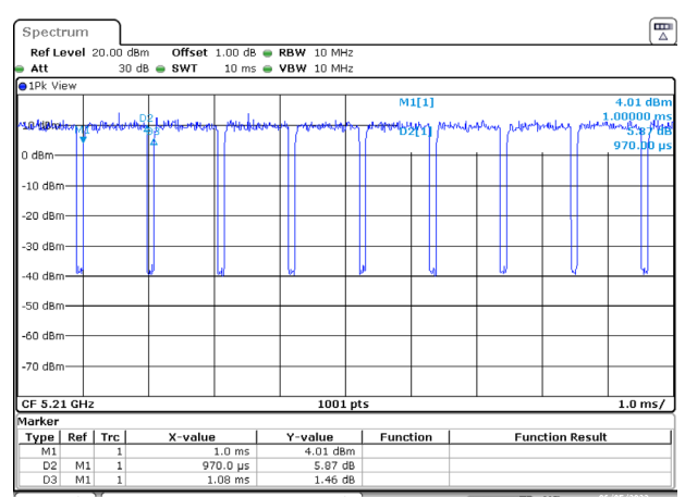
802.11ax-80 MHz
