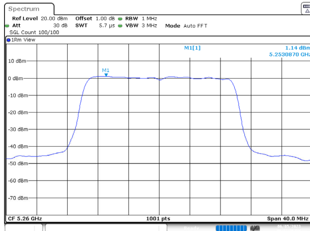
Channel 52
