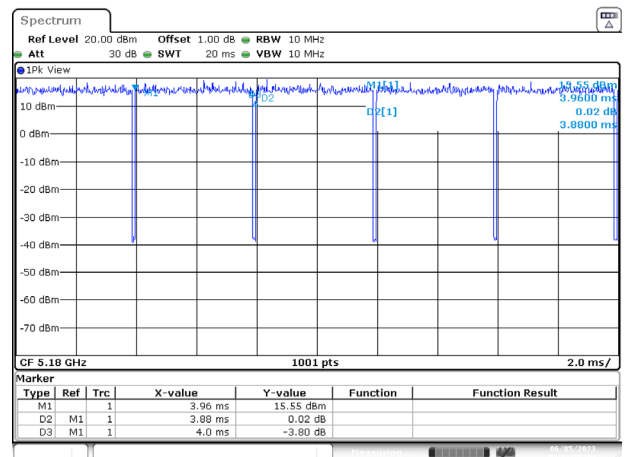
802.11ax-20 MHz
