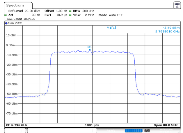
Channel 159
