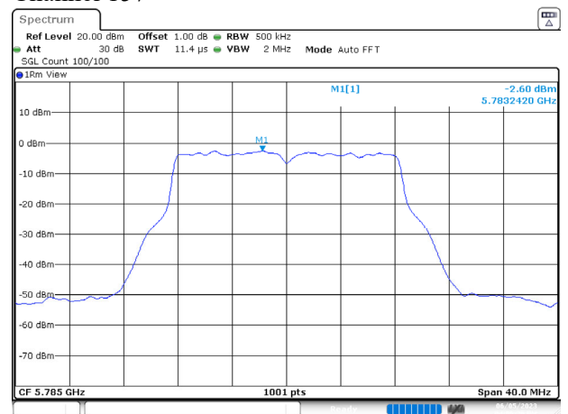
Channel 157
