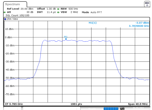
Channel 157
