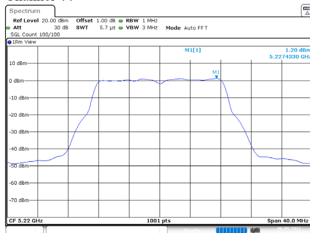
Channel 44
