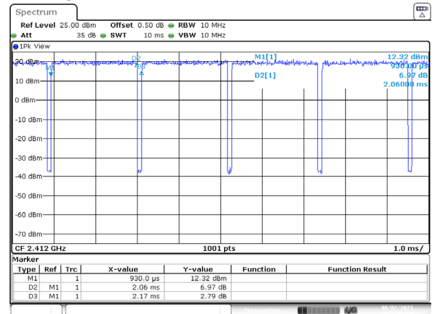
802.11g
