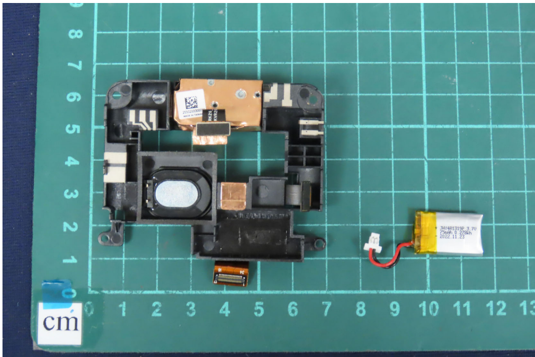
(27) EUT Photo
