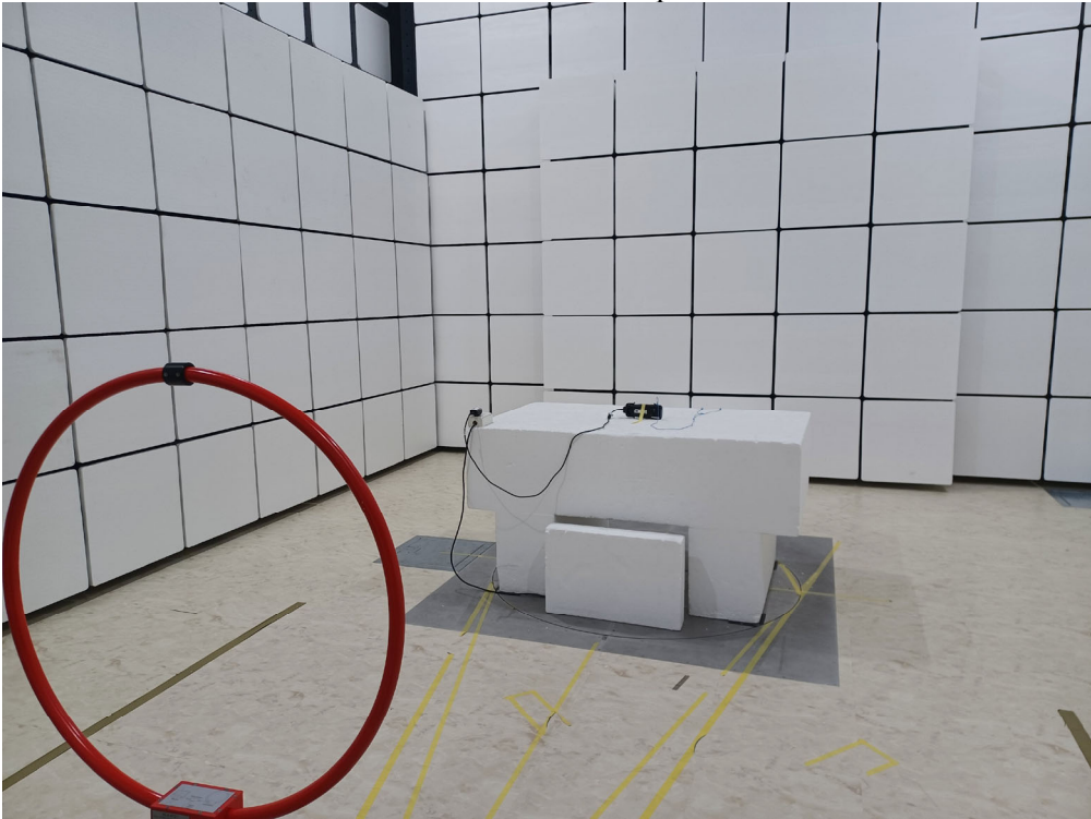
Radiated Test-Loop
