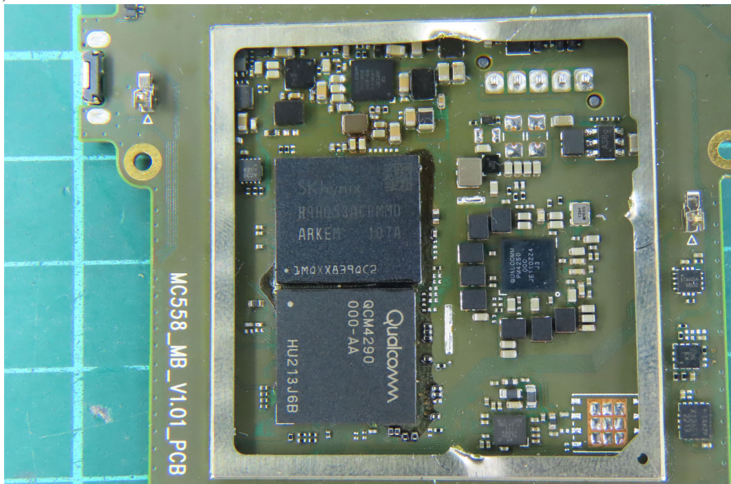
(42) EUT Photo
