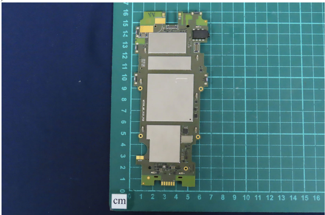
(38) EUT Photo
