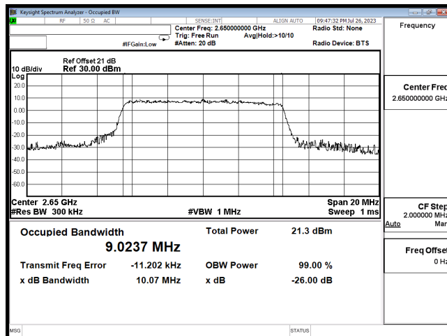
OCC B41 10M CH41190 64QAM
