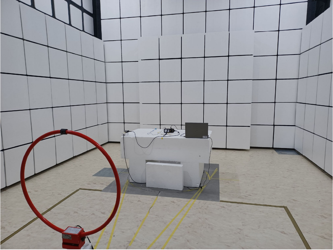
Radiated Test-Loop
