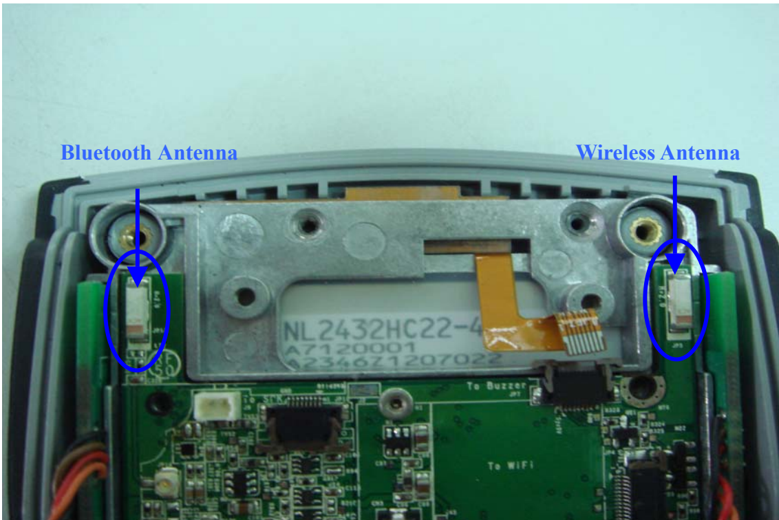
For Wireless & Bluetooth Antenna (Multilayer Chip Antenna)
