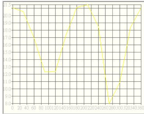
PCS Ch. 810@Theta 30.0 Vertical Excel XY Plot
