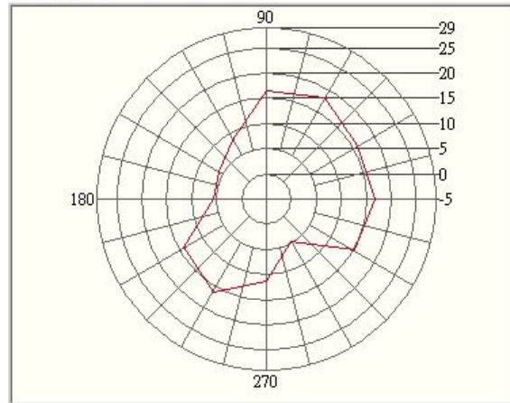
PCS Ch. 810@Theta 60.0 Vertical Excel XY Plot
