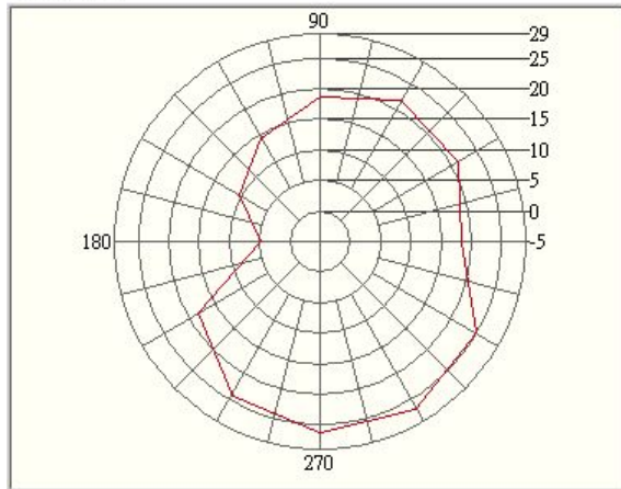
PCS Ch. 810@Theta 60.0 Horizontal Excel XY Plot
