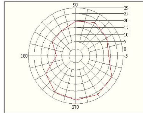
PCS Ch. 661@Theta 60.0 Total Excel XY Plot
