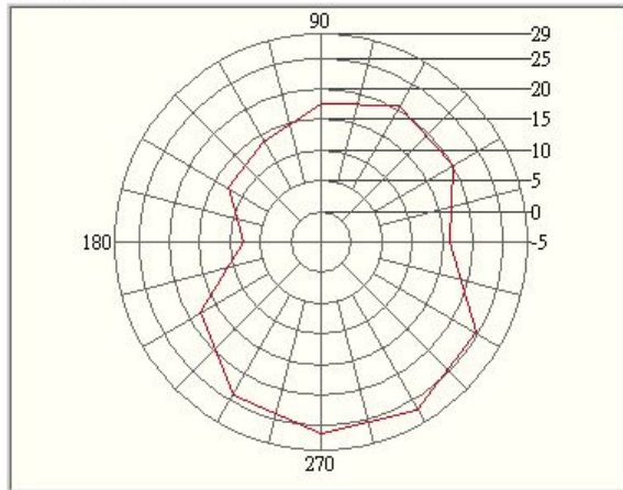
PCS Ch. 661@Theta 60.0 Horizontal Excel XY Plot
