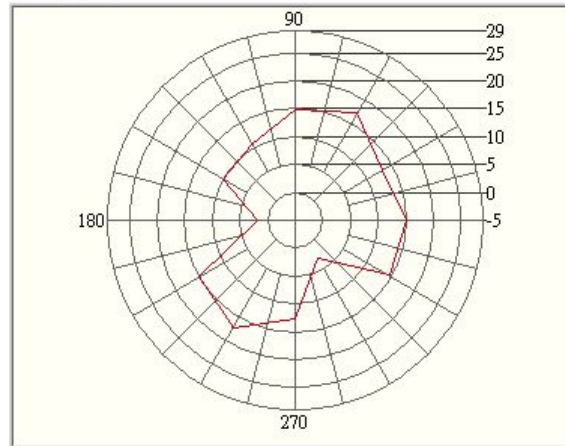
PCS Ch. 661@Theta 60.0 Vertical Excel XY Plot
