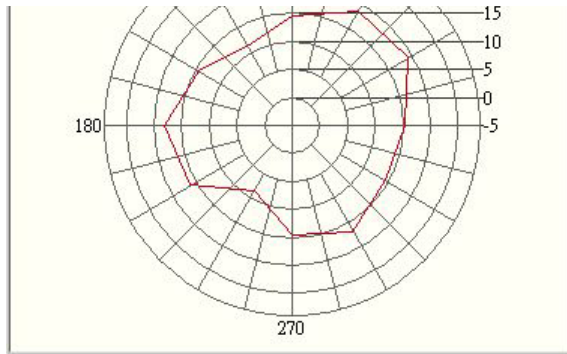
PCS Ch. 810@Theta 120.0 Worksheet1 Excel XY Plot
