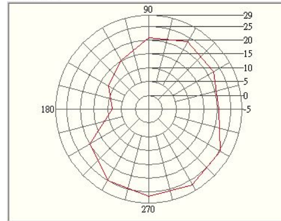
PCS Ch. 810@Theta 60.0 Total Excel XY Plot
