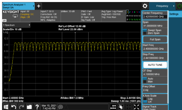
3-DH5(3Mbps)-2400~2441MHz
