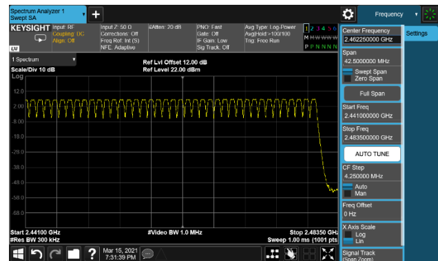
3-DH5(2Mbps)-2441~2483.5MHz
