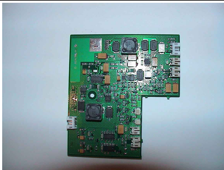
Supply PCB
