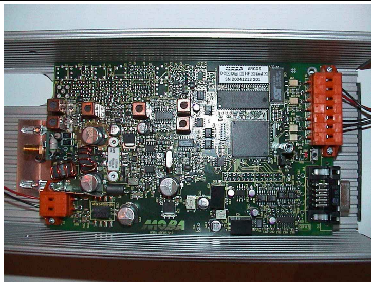
RF-PCB in central unit
