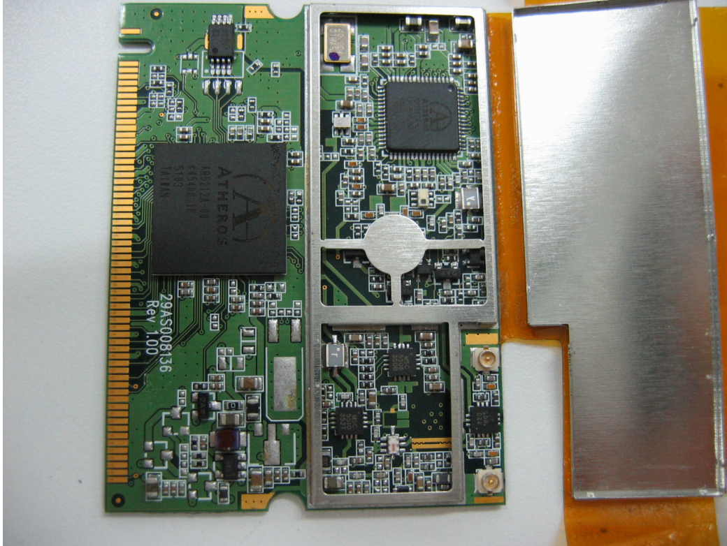
Photograph No.6 Winlink 1000/F49 RF board
