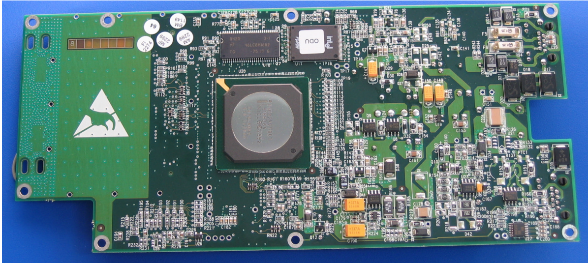
Photograph No.5 Winlink 1000/F49 Main PCB second side view
