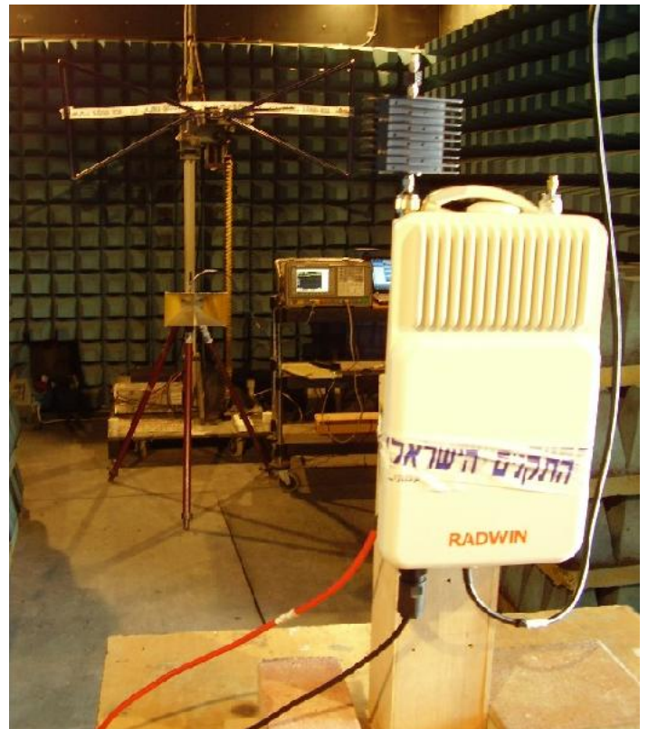
Photo #3. Radiated emissions test setup in anechoic chamber.
