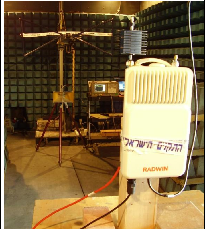
Photo #4. Radiated emissions test setup in anechoic chamber.
