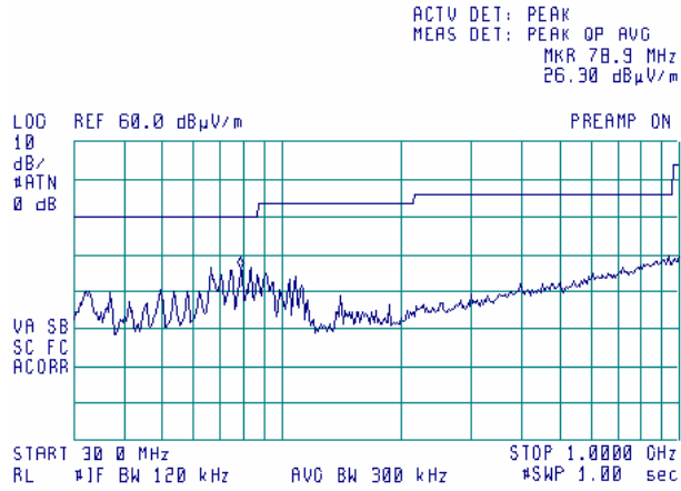
Plot 7.4.110 Radiated emission measurements from 30 to 1000 MHz at the low carrier frequency
