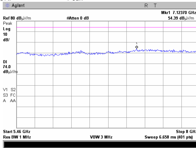
Plot 7.3.55 Radiated emission measurements from 5.46 to 8.0 GHz at the low carrier frequency
