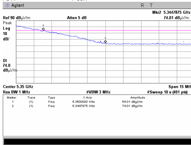
Plot 7.4.16 Radiated spurious emission measurements at the band edges
