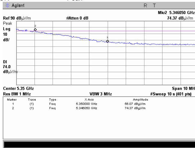
Plot 7.4.40 Radiated spurious emission measurements at the band edges
