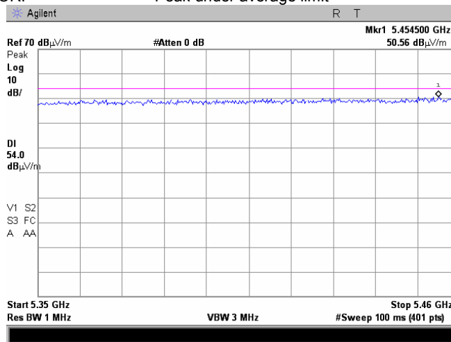
Plot 7.3.51 Radiated emission measurements from 5.35 to 5.46 GHz at the mid carrier frequency
