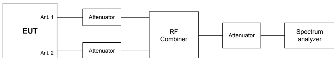
Figure 7.4.2 Spurious emission test setup– combined Tx chains
