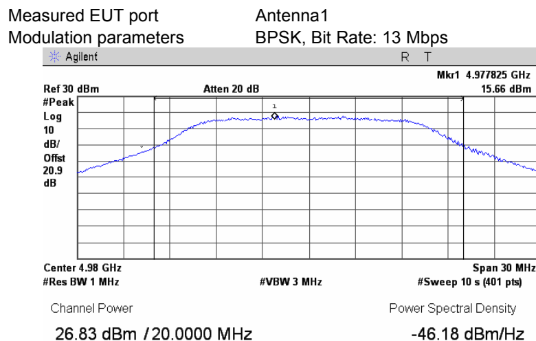
Plot 7.1.30 Peak output power test results at high frequency
