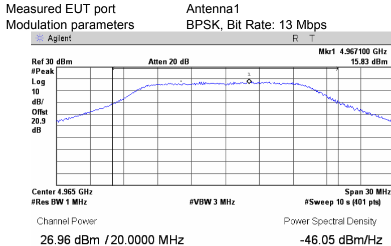
Plot 7.1.29 Peak output power test results at mid frequency
