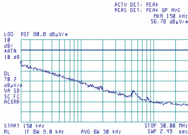
Plot 7.5.6 Radiated emission measurements in 0.15 - 30 MHz range
