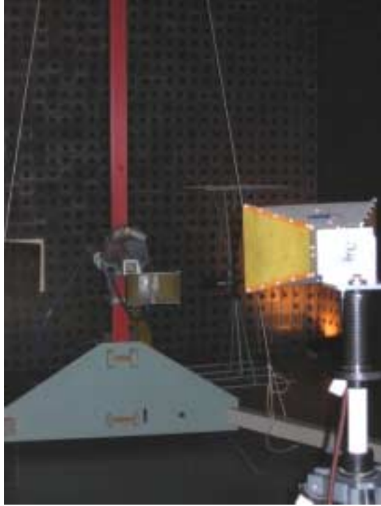
Photograph No.8 Substitution ERP measurements of spurious setup in the anechoic chamber
