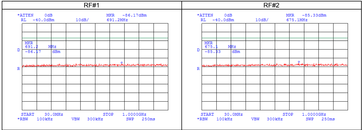
Plot 7.12.1 Spurious emission test results
