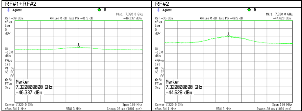
Plot 7.6.19 Spurious emission measurements at the 2 nd harmonic of low carrier frequency
