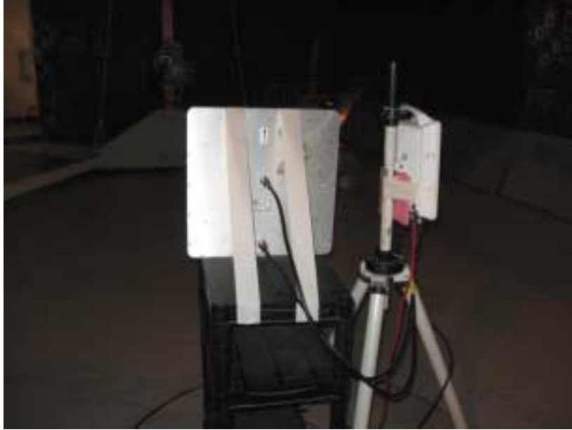
Photograph No.9 EUT with external antenna setup in the anechoic chamber
