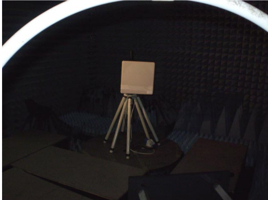
Photograph No.5 Radiated emissions measurement setup in the anechoic chamber with loop antenna
