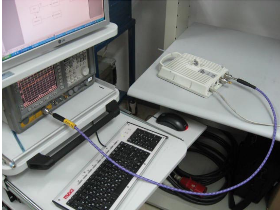
Photograph No.11 Receiver spurious emissions measurement setup
