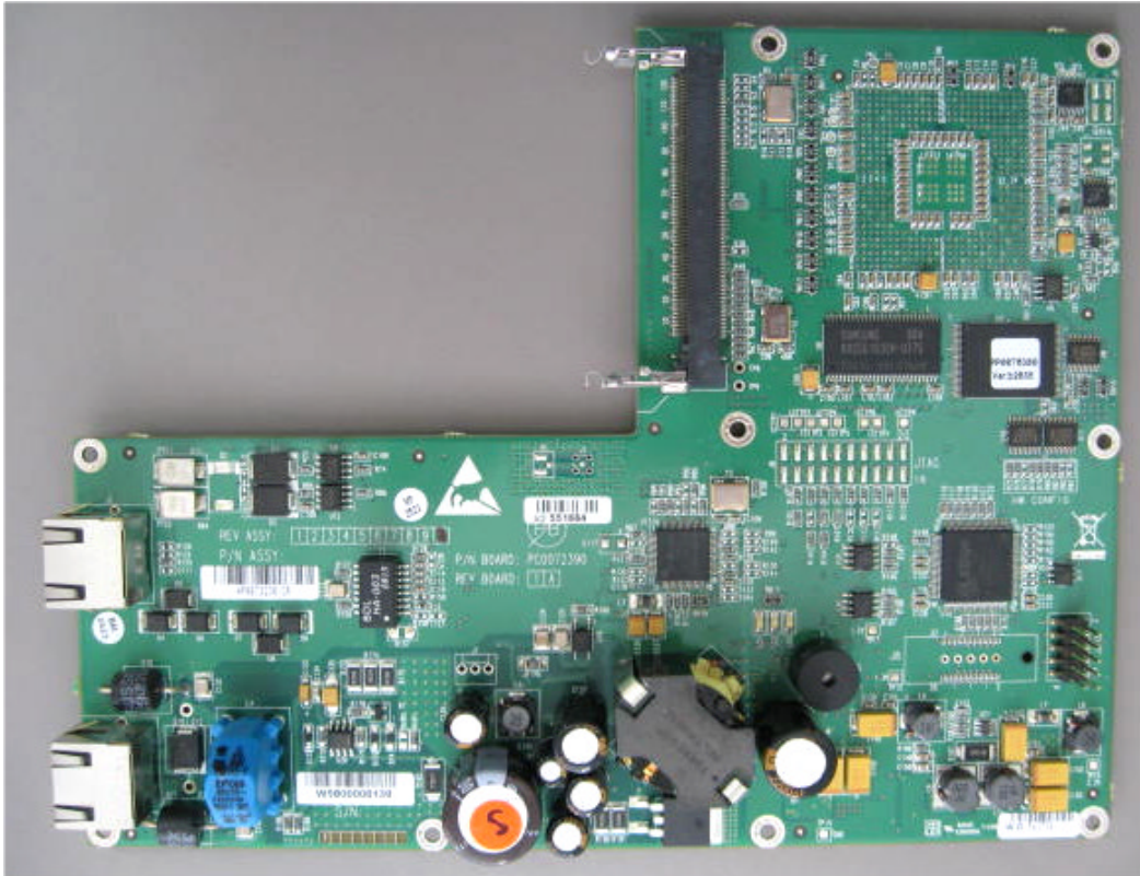
Photograph No6 RADWIN 1000/2000 main PCB front view
