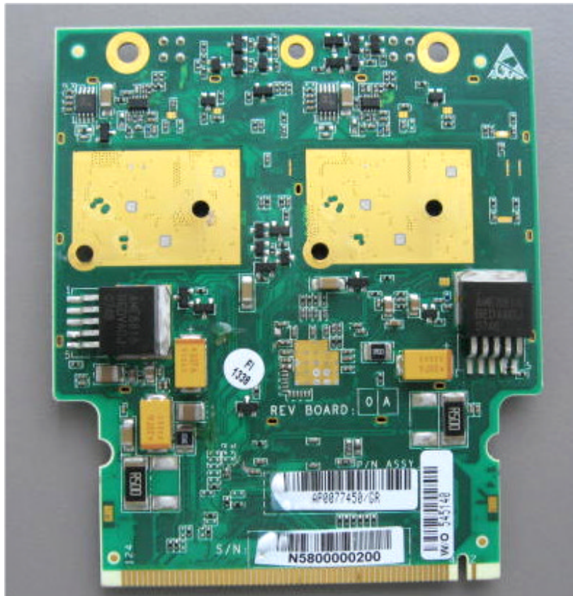
Photograph No9 RF module second side of RADWIN 1000/2000
