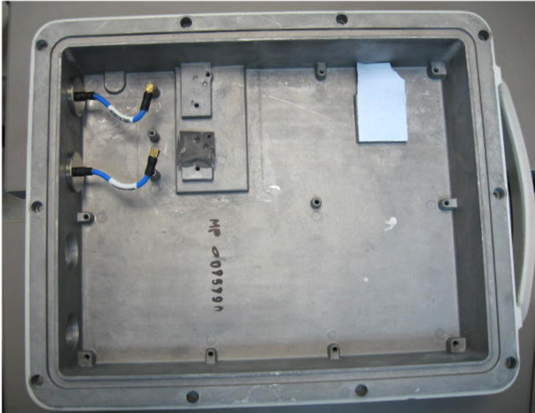
Photograph No3 RADWIN 2000 case internal view
