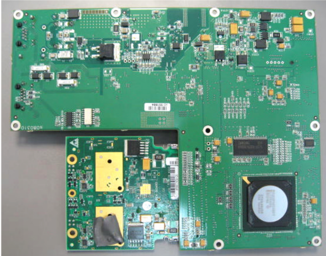
Photograph No5 RADWIN 1000/2000 main PCB with RF card second side view
