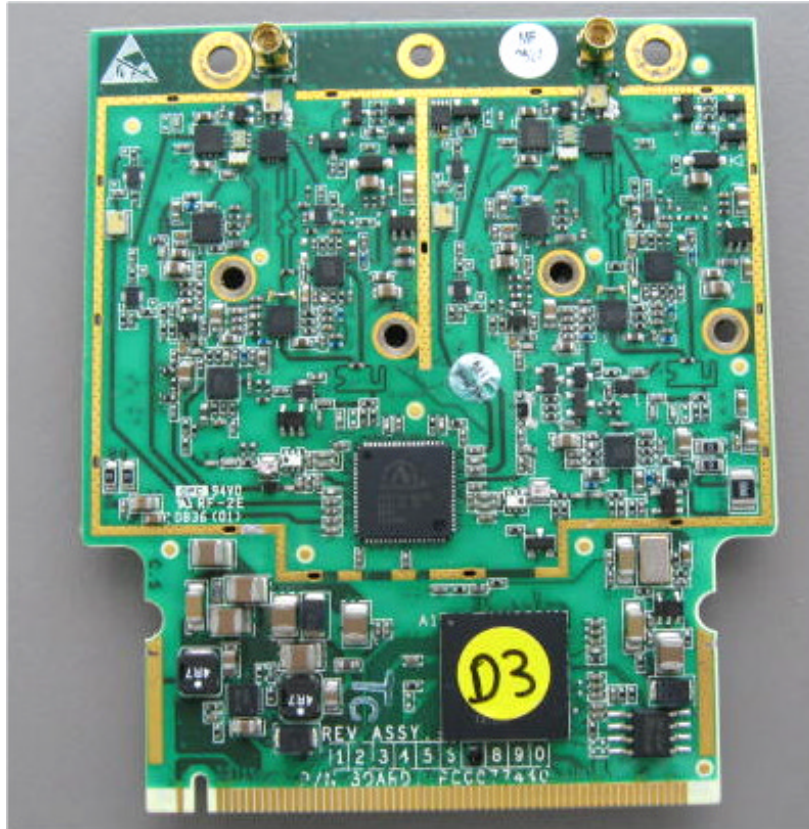
Photograph No8 RF module of RADWIN 1000/2000 front view
