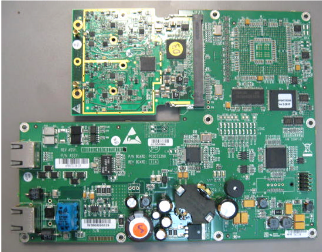
Photograph No4 RADWIN 1000/2000 main PCB with RF card front view
