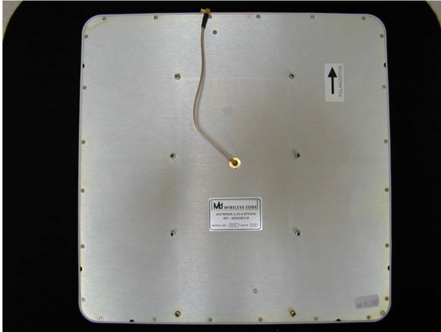
Integral antenna
