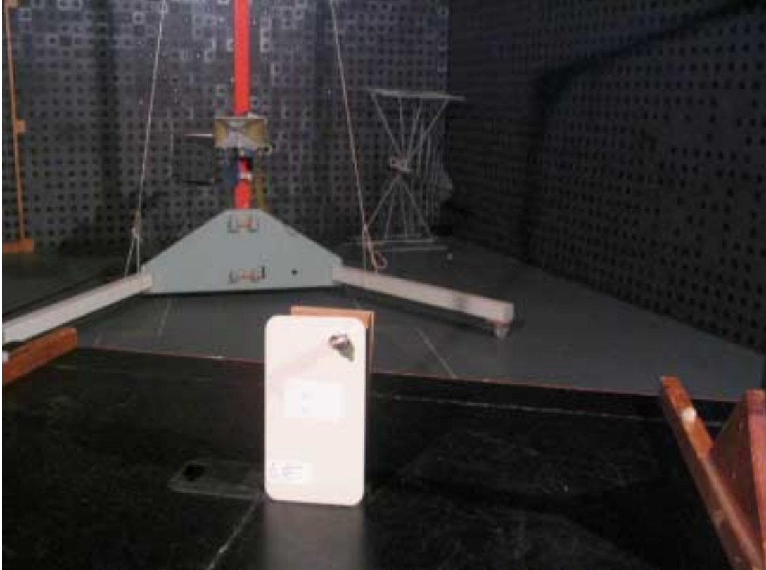
Photograph No.4 Radiated emissions measurement setup in the anechoic chamber with horn antenna
