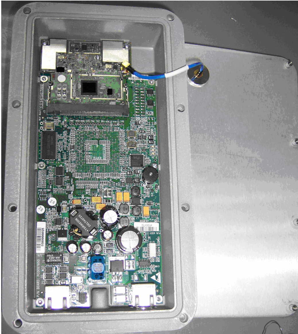
Photograph No.1 Winlink 1000-HE/F25/BRS (ODU) internal view
