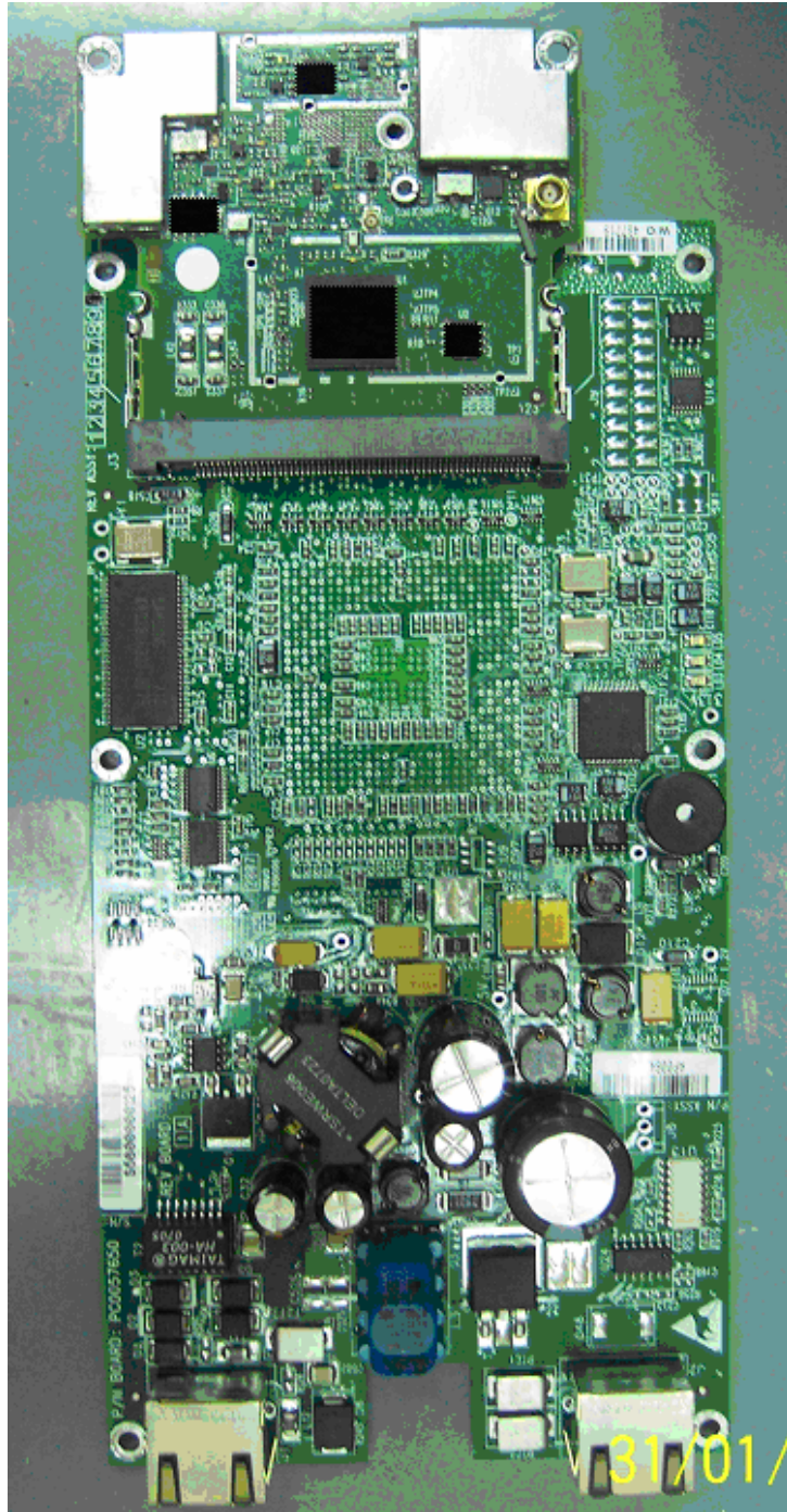
Photograph No.4 Winlink 1000-HE/F25/BRS (ODU) PCB front view
