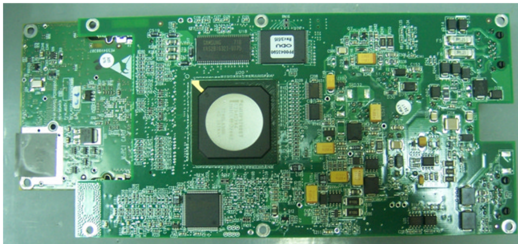
Photograph No.5 Winlink 1000-HE/F25/BRS (ODU) PCB second side view
