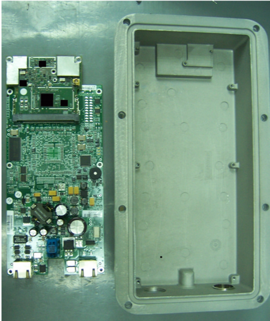
Photograph No.3 Winlink 1000-HE/F25/BRS (ODU) internal view, PCB removed from the case
