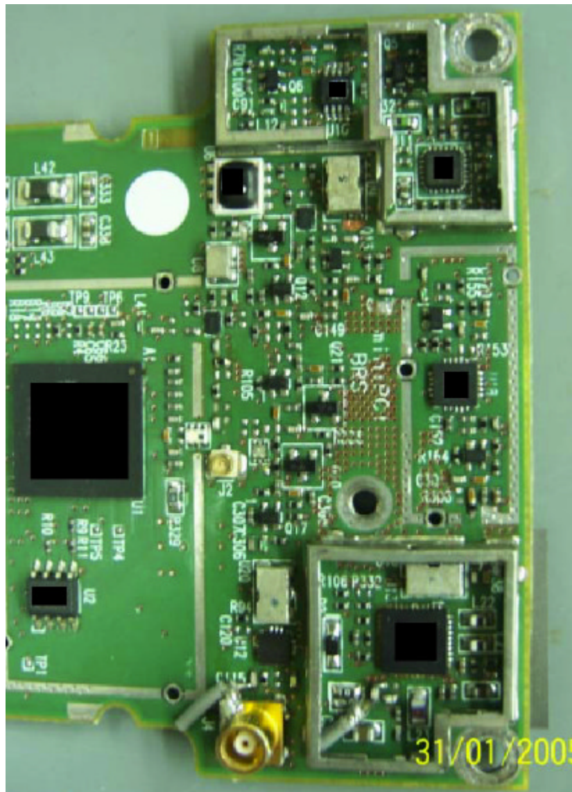
Photograph No.10 RF module with shields removed
