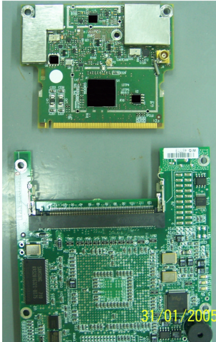
Photograph No.7 ODU PCB with RF module removed
