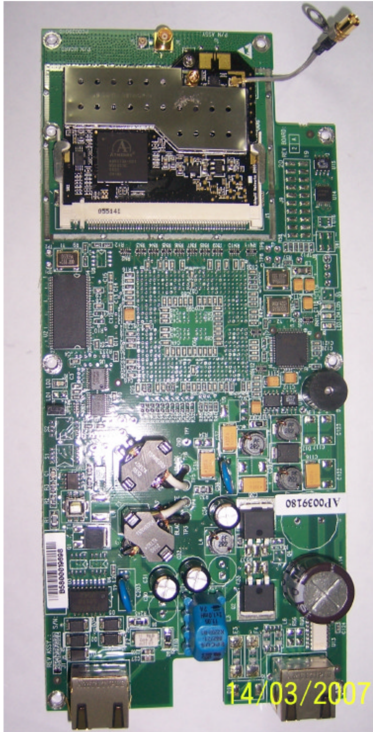
Photograph No.3 WinLink 1000/F24/HE main PCB front view
