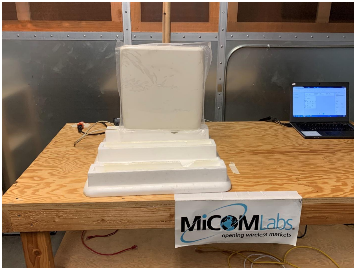
RDWN69 AC Conducted Emissions front view
