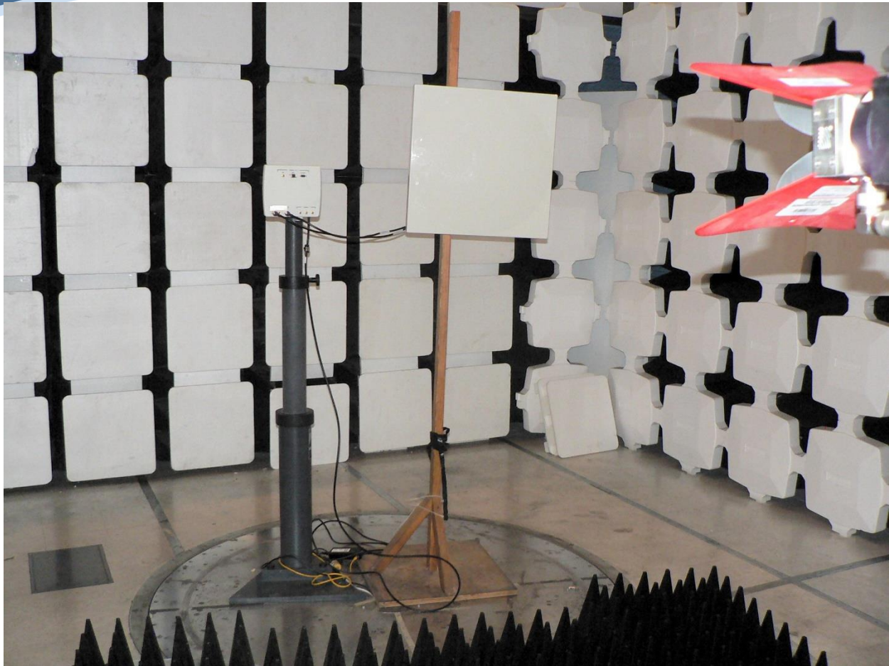
Tx Spurious 28 dBi Panel
