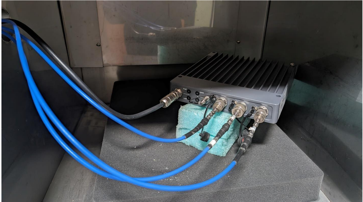
Conducted RF
