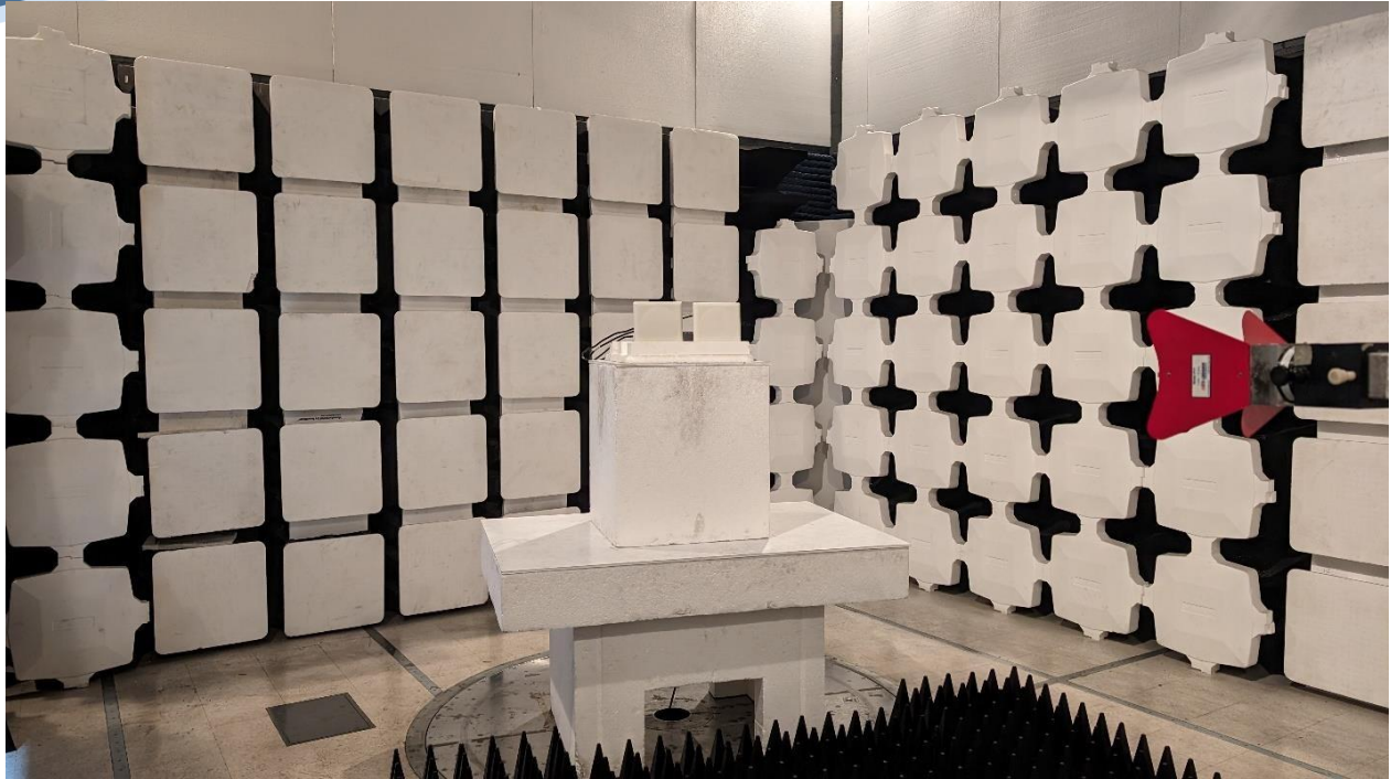
Spurious Emissions RW-9105-5158
