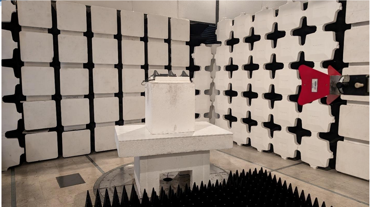
Spurious Emissions RW-9401-5004
