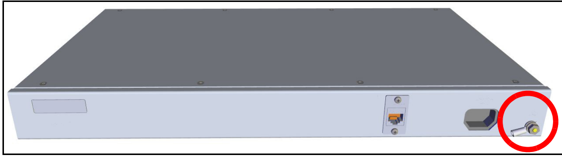
Figure 2-98: ISU: Grounding lug location
