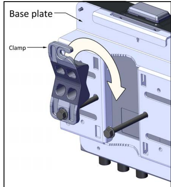
Figure 2-8: Thin pole: Do not completely tighten bolts
