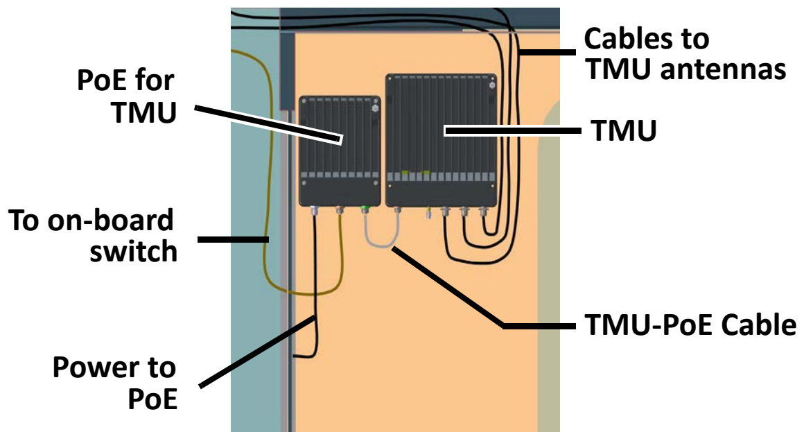
Figure 2-69: On-board general mounting arrangement - detail view
