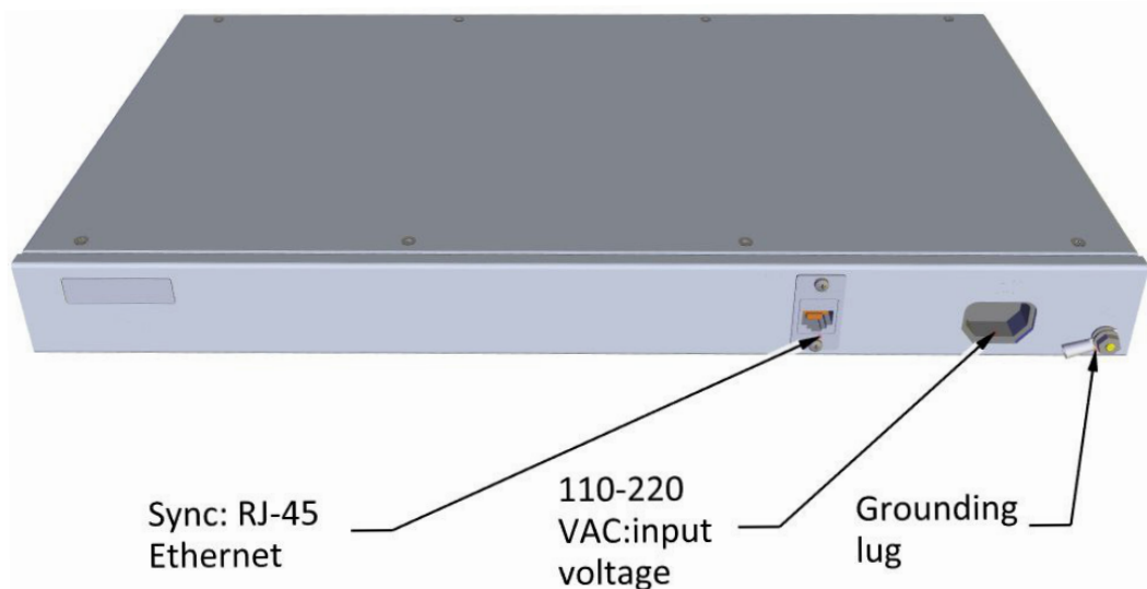
Figure 2-53: Indoor Synchronization Unit (ISU)
