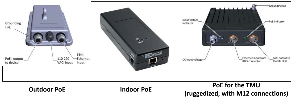
Figure 1-11: PoE Units
