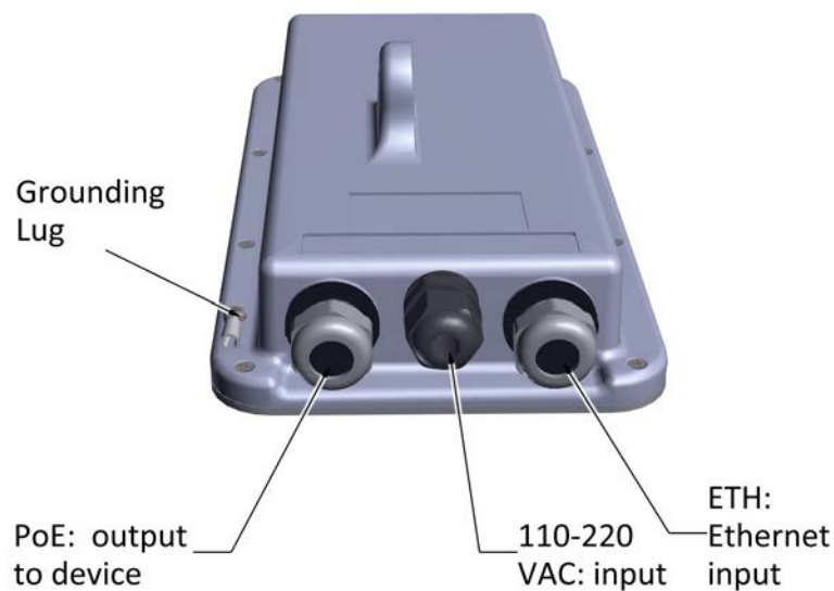
Figure 2-35: PoE external connections
