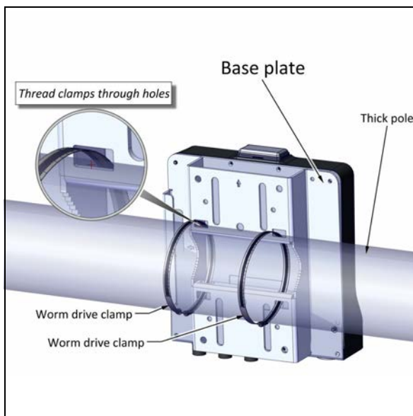
Figure 2-28: Using metal bands for a large pole Figure 2-29: Using U-bolts for a large pole
