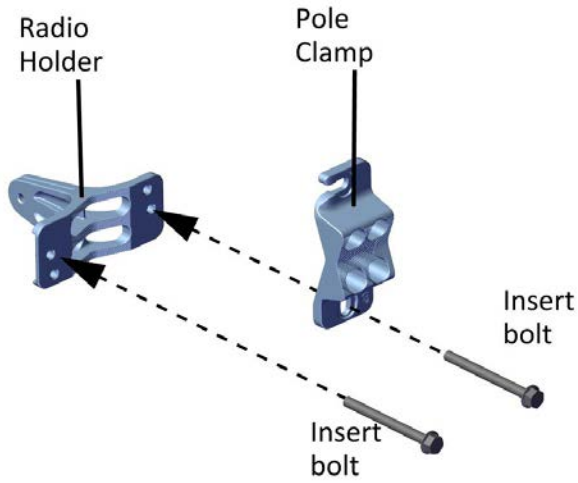
Figure 2-41: Connect Pole Clamp to Radio Holder
