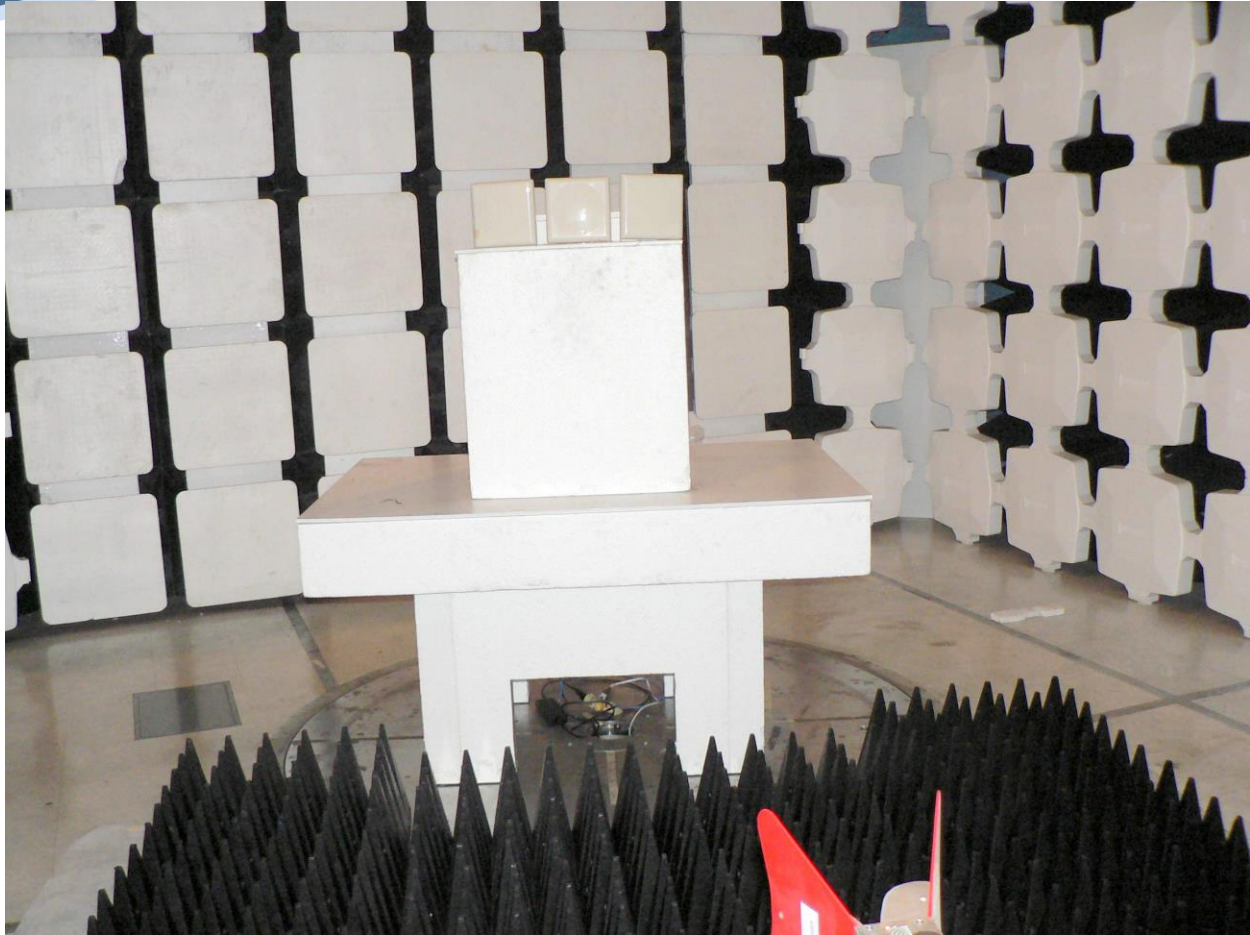
RDWN63 TX Spurious AT0058760 Antenna
