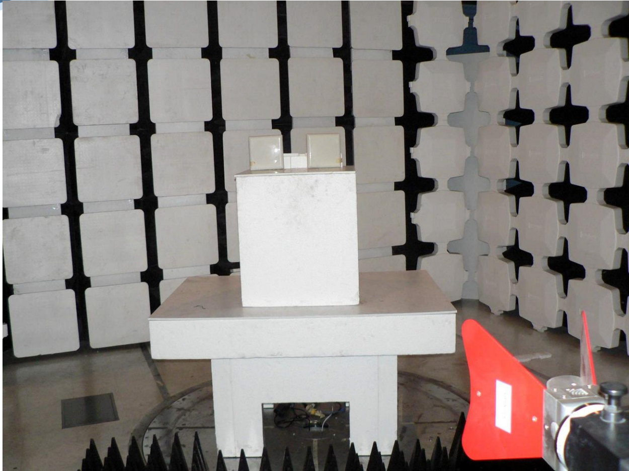
RDWN63 Tx Spurious RW-9105-5158 Antenna
