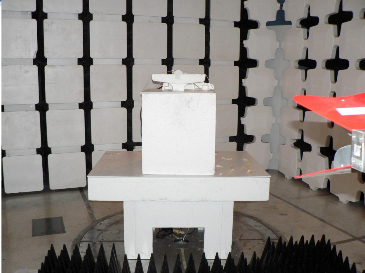
RDWN63 Tx Spurious RW-9314-5158 Antenna
